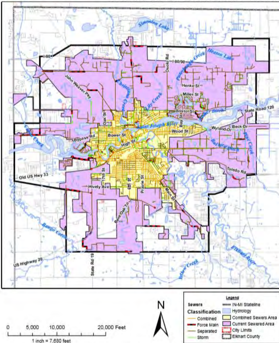
Figure 9-2 Combined Sewer Areas
