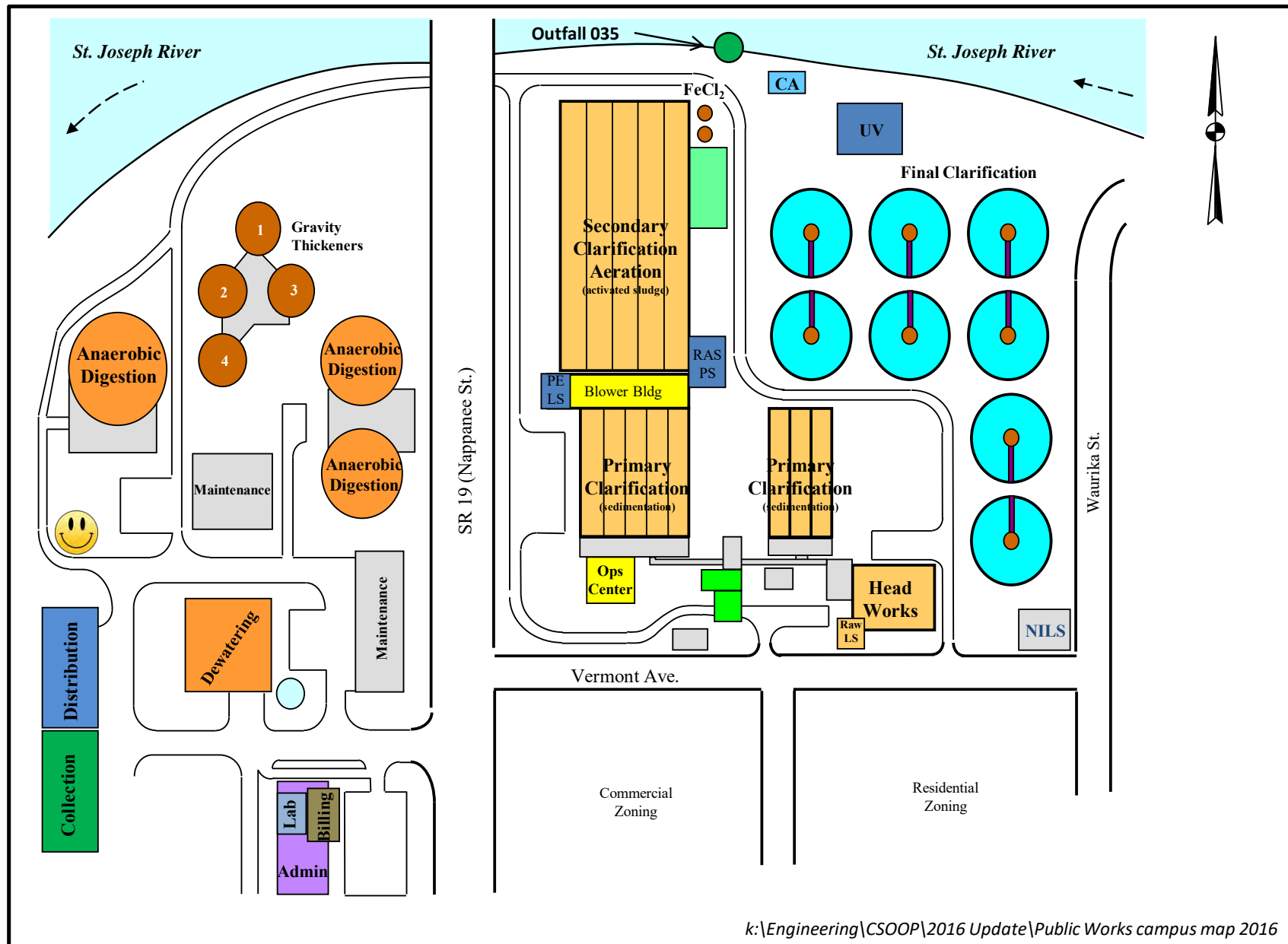
Figure 1-5 Elkhart Wastewater Treatment Plant
